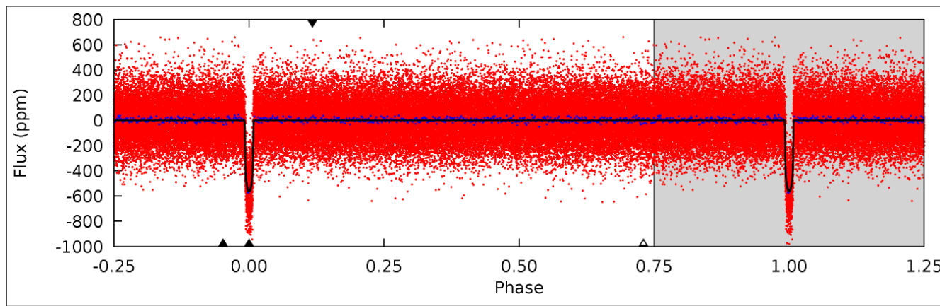
Figure 21: The red points show the phased photometric light curve (in this case the DV detrending) for the candidate event. Blue points show binned data, such that eight binned points lie within the primary transit. In this example, as it is a high SNR planet candidate, the blue points mostly all lie behind the black model line. The black line shows the best-fit transit model (in this case the DV model). The primary event is located at phase zero and is marked by an upward-facing triangle on the bottom axis. The other triangles mark the locations of potential secondary (filled) and tertiary events (open); the location of the strongest anti-transit (positive event) is marked by the downward-facing triangle on the top axis. The grayed out area from phase 0.75 to 1.25 plots the same data as is plotted between phases -0.25 and 0.25.
