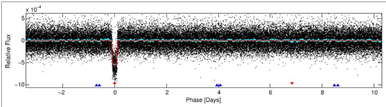
Figure 4: The photometric data folded at the orbital period of the candidate transit event. The red line shows the best-fit transit model. The blue-circled, cyan-filled points show the data binned. The transit event is located at phase 0.0 and marked with an upward-facing, red triangle. The downward-facing, red triangle marks the location of the strongest secondary event via the weak secondary test. Upward-facing triangles of other colors show the locations of the primary events of other TCEs in the system, in the phase space of the current TCE under examination.
